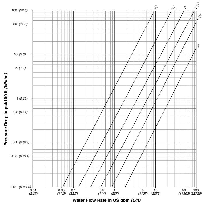
Chart settings at 120°F (49°C)
