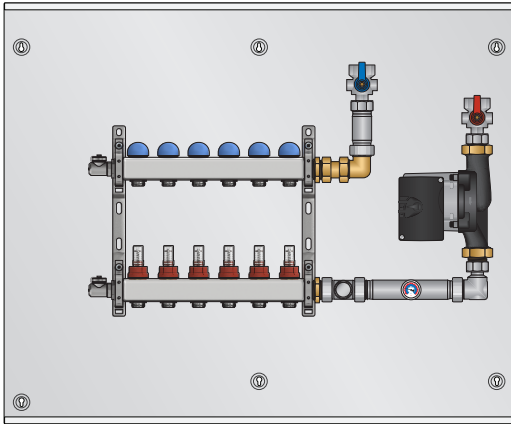
SSPLx10xT - Large (26-99) pump, mixing valve, 76100 manifold with flow meters (shown with 6 loops), top feed.
