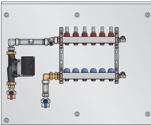
SSPLx10xB - Large (26-99) pump, mixing valve, 76100 manifold with flow meters (shown with 6 loops), bottom feed.
