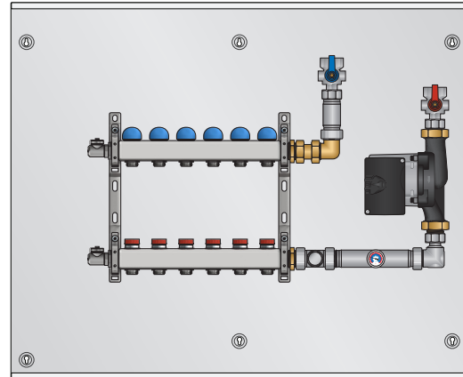
SSPLx20xT - Large (26-99) pump, mixing valve, 76200 high flow manifold (shown with 6 loops), top feed.
