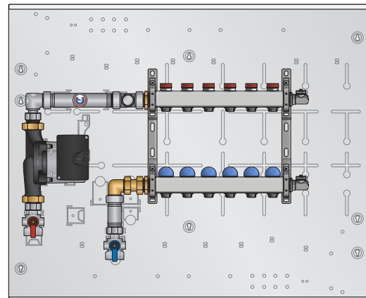
SSPLx20xB - Large (26-99) pump, mixing valve, 76200 high flow manifold (shown with 6 loops), bottom feed.
