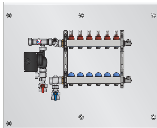
SSPSx10xB - Small (15-58) pump, mixing valve, 76100 manifold with flow meters (shown with 6 loops), bottom feed.
