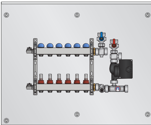
SSPSx10xT - Small (15-58) pump, 3-way mixing valve, 76100 manifold with flow meters (shown with 6 loops), top feed.
