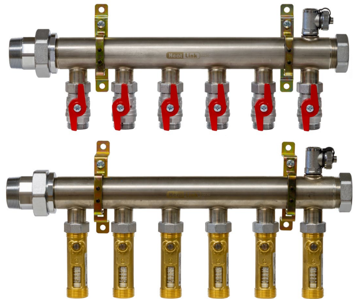
76706 - 6 loop model
