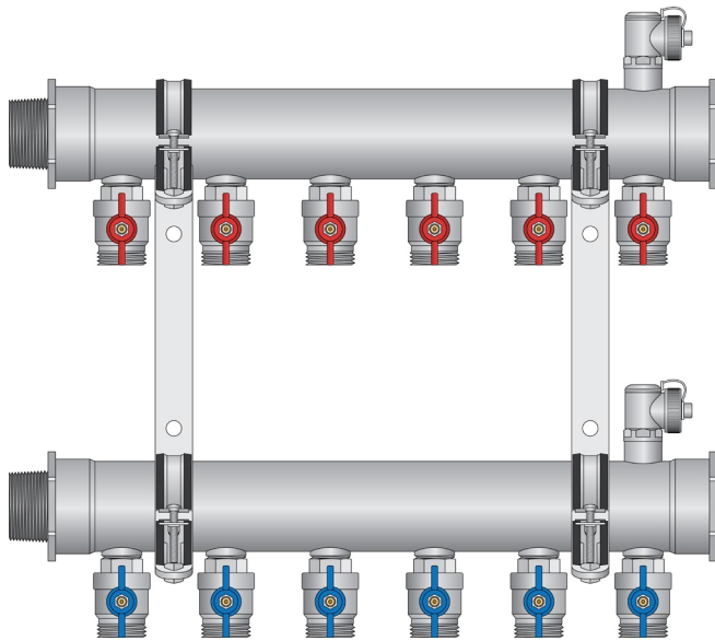
76606 - 6 loop model with 76840 - 1-1/2" assembly kit
