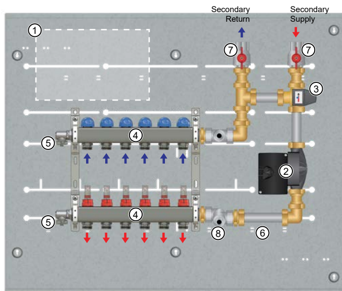
SSTV with UPS 15-58 pump, 75106 manifold, top feed mains.
